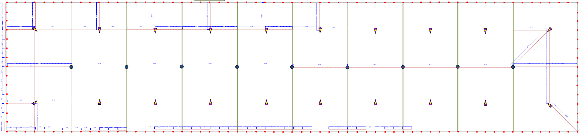
70' x 310' Pole Tent - Pole Placements Blue dots = Center pole position Red dots = side pole positions Green Line indicates Lace Line locations Triangles indicate Quarter Pole locations
